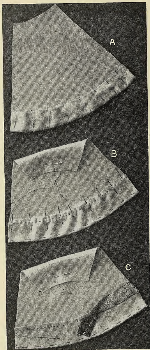
FIG. 213.—Finish for lower edge of wool skirt; A, hem turned and pinned; B, fulness drawn up by gathers; C, fulness shrunk out and Prussian binding basted to hem.
